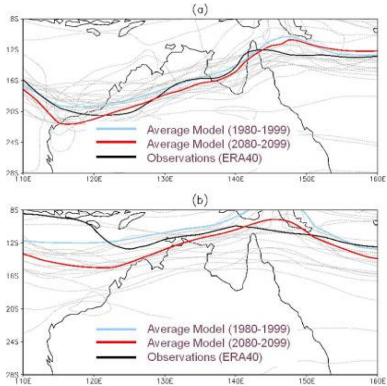
Figure 21: Monsoon ‘shearline’ during the 1980–1999 period (OBS and CMIP3 ensemble mean) and during the 2080–2099 period (CMIP3 ensemble mean). Shown are January (a) and March means (b).
