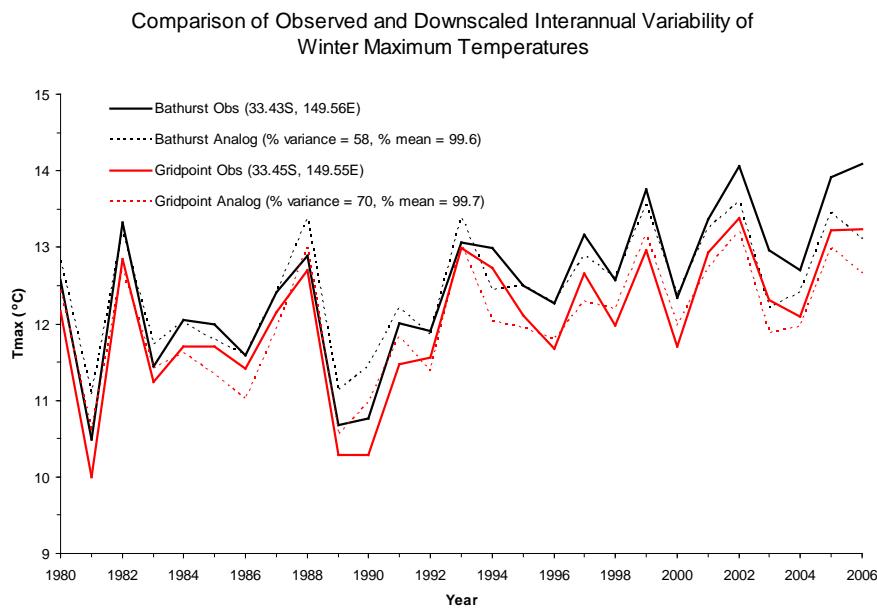
Figure 25: Comparison of the observed (solid curve) and downscaled (dashed curve) year-to-year variability of mean winter maximum temperatures. The red curves denote the observed and downscaled variability of the grid point data located close to the Bathurst observation stations (black curves).
