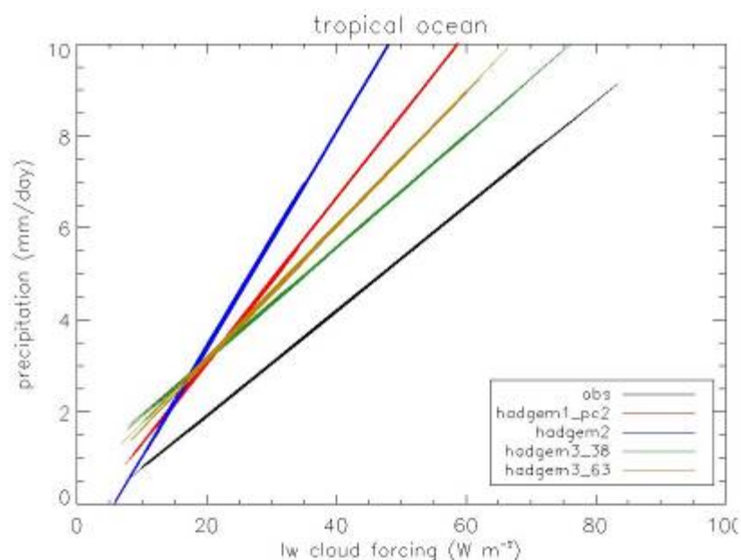
Figure 18: Relationship between long wave cloud-forcing and precipitation-rates over tropical-ocean points. Black – observations, Red – HadGEM1+PC2, Blue – HadGEM2, Green – HadGEM3 38 Levels, Brown – HadGEM3 63 Levels.
