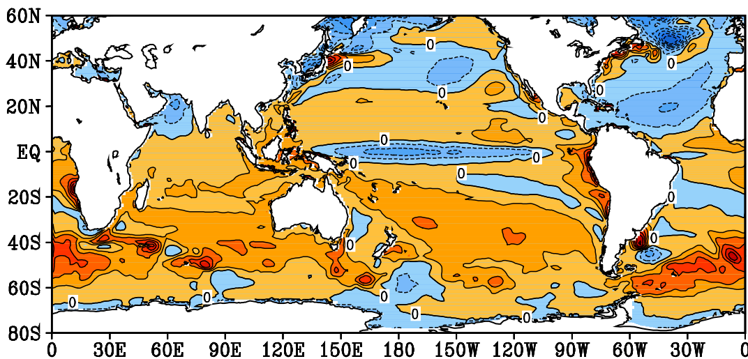
Figure 16: Difference in sea surface temperature between model (years 71–100 of Expt. 5) and observations (according to HadSST data set).
