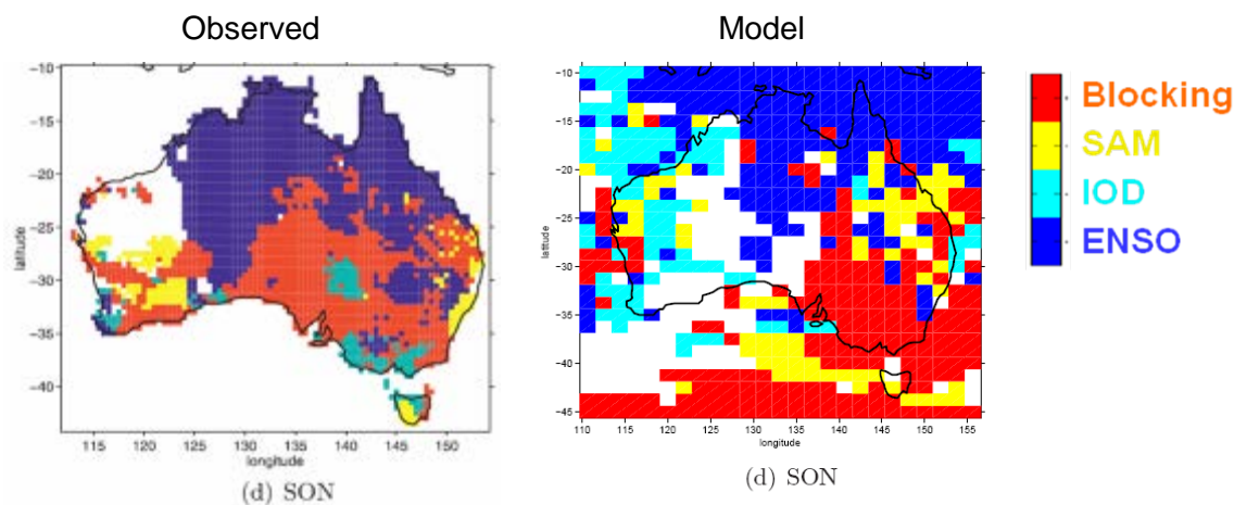
Figure 17: Patterns of influence of four remote drivers of Australian rainfall (blocking over the southern Tasman Sea, the Southern Annular Model (SAM), Indian Ocean Dipole (IOD) and ENSO). Colours on maps indicate the dominant driver (in terms of strongest correlation) at each location. Model result is from an ACCESS atmospheric model simulation over the years 1979–2008.
