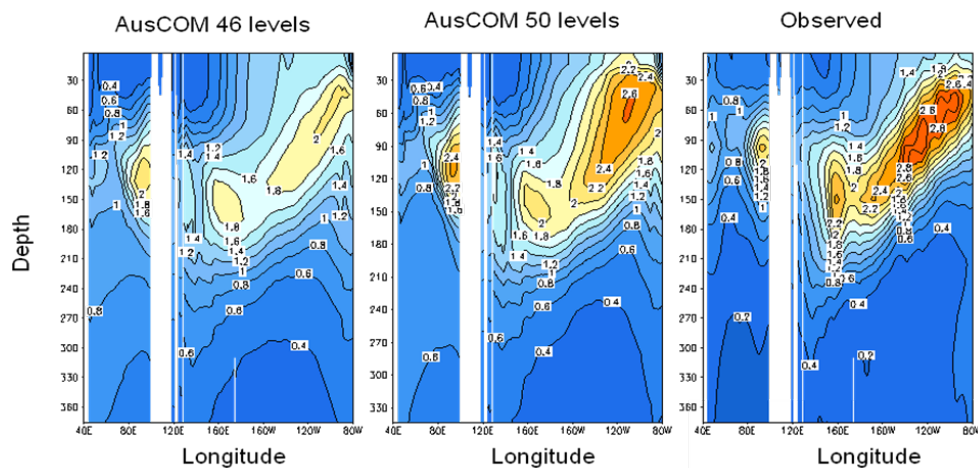
Figure 19: Comparison of standard deviation of temperature anomaly along equator from 40°E to 80°W over the period 1980 to 2005 of AusCOM model with the previously standard lower resolution over the depth range 50-200 m (left), AusCOM model with higher resolution over that depth range (centre), and observations (right). Units are °C.
