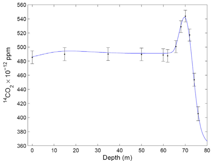
Figure 3: ‘Nuclear bomb pulse’ of 14 CO 2 measured in NEEM firn air (Greenland) and model prediction, to use as dating constraint
