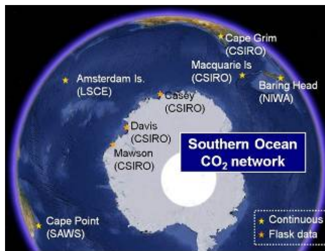
Figure 1: Southern Ocean region collaborative CO 2 observation network
