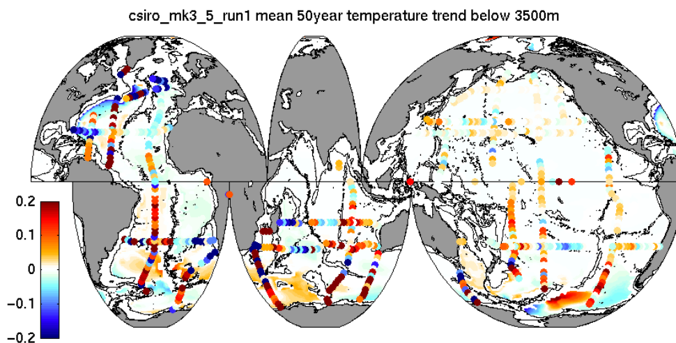
Figure 11: Comparison of the 50 year temperature trend between a global climate model (colour contour) and observations (colour dots) below 3500 m
