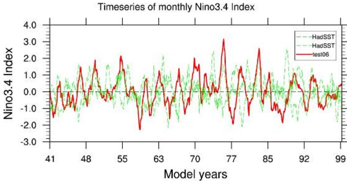
Figure 15: Time series of sea surface temperature anomaly in the Nino3.4 area (5° N–5° S; 120° W–165° W) for years 41-100 of ACCESS Test 6 (red) and observed according to two representative time slices from the HadSST data set (green).
