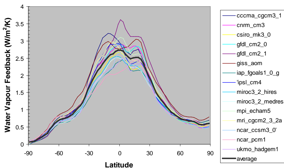
Figure 13: Structure of water vapour feedbacks in a range of the AR4 models as a function of latitude. Feedback units are watts/square metre per Kelvin of global warming. Also shown is the average of all the models (heavy black line). This plot shows that both the magnitude of the water vapour feedback and the differences in feedback strength between models is dominated by the tropics (i.e. to roughly 30° north and south). Models also show differences in their latitude of maximum feedback, and a tendency to have more than a single low latitude ‘peak’. Further analysis shows this to be due to the effect of cloud ‘shielding’ on water vapour feedback.
